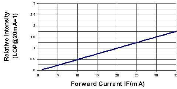
Relative Luminous Intensity vs Forward Current
