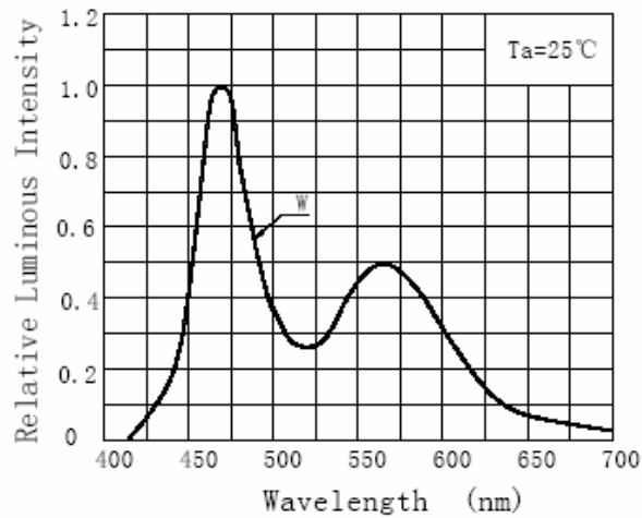
Relative Luminous Intensity VS Wavelength
